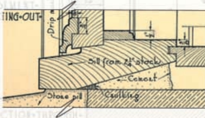
above: INSET C SAMPLE OF DOUBLE STEPPED SILL
